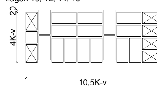
Lagen 10, 12, 14, 16
